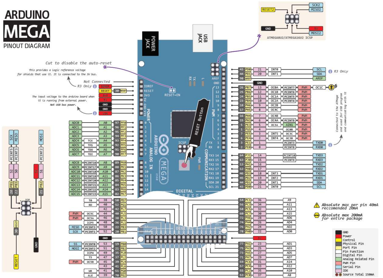
Figure 7.3. Arduino Mega
